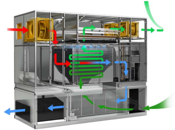
Internal arrangement of ATP as deployed
